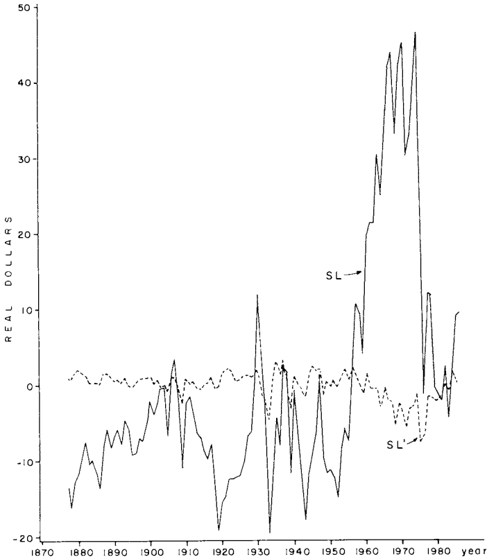
Fig. 2.—Stock market: deviations from means of actual spread ( SL_t = Price_t - \theta \cdot Dividend_{t-1} ) and theoretical spread SL'_t , \theta = 12.195 .
