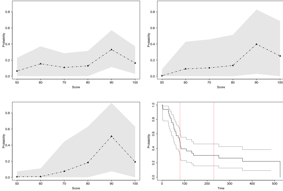
Figure 8: From top left: pmf prediction at 70, 230 and 550 days after the experiment. Bottom right: Kaplan-Meyer estimate of the survival times up to time 550.
