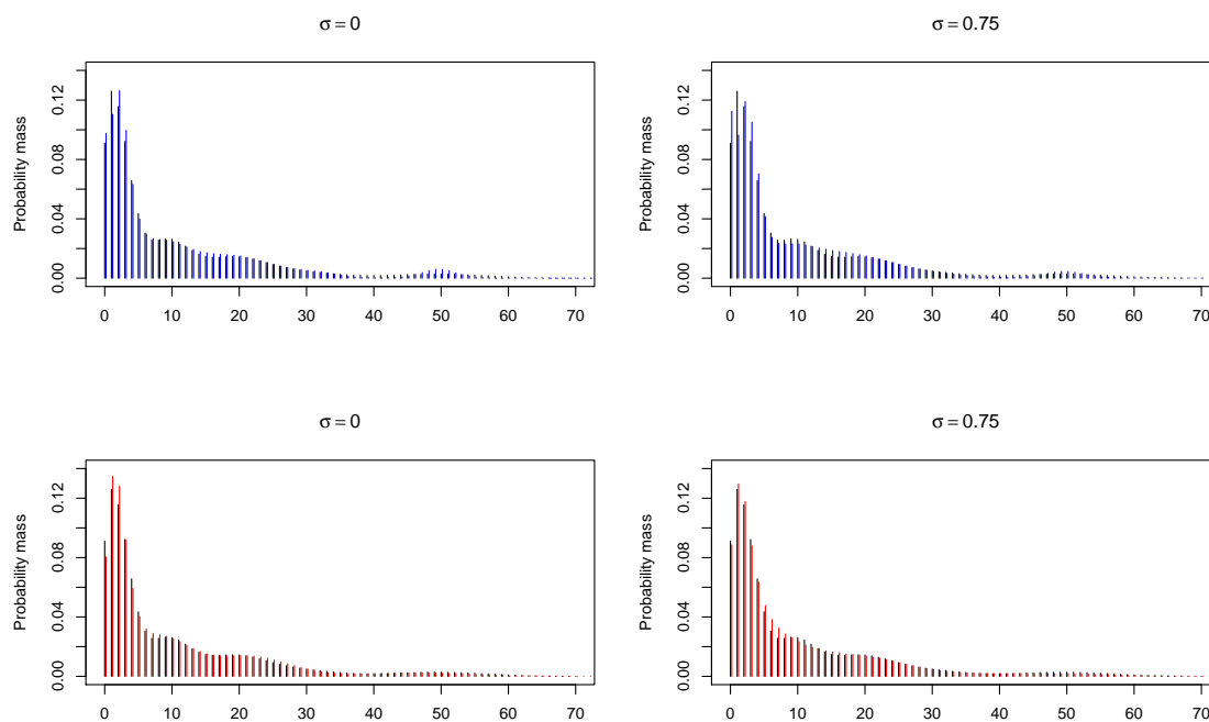
Figure 13. Posterior probability mass functions given n = 200 data generated from the 6 component Poisson mixture. The first row displays the posterior estimates of the RG model (depicted in solid blue) whereas the second of the Poisson model (depicted in solid red) both with \mathbb{E}[K_n] = 6 and, respectively, \sigma = 0 and \sigma = 0.75 . The true pmf are in solid black.
