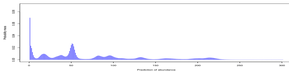
(b) \sigma = 0.25
