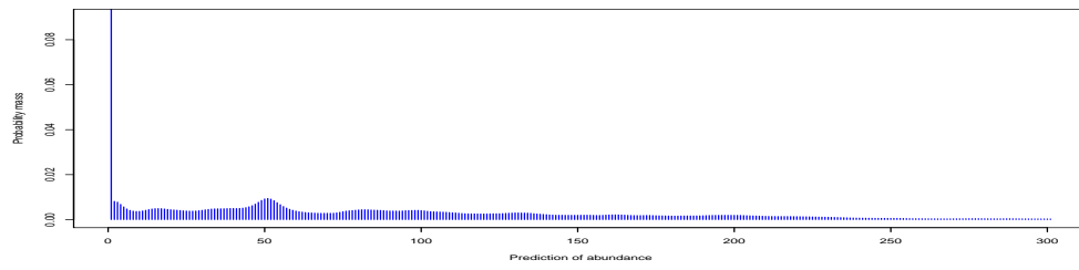
(b) \sigma = 0.25
