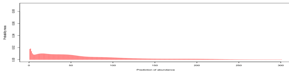
(a) \sigma = 0
