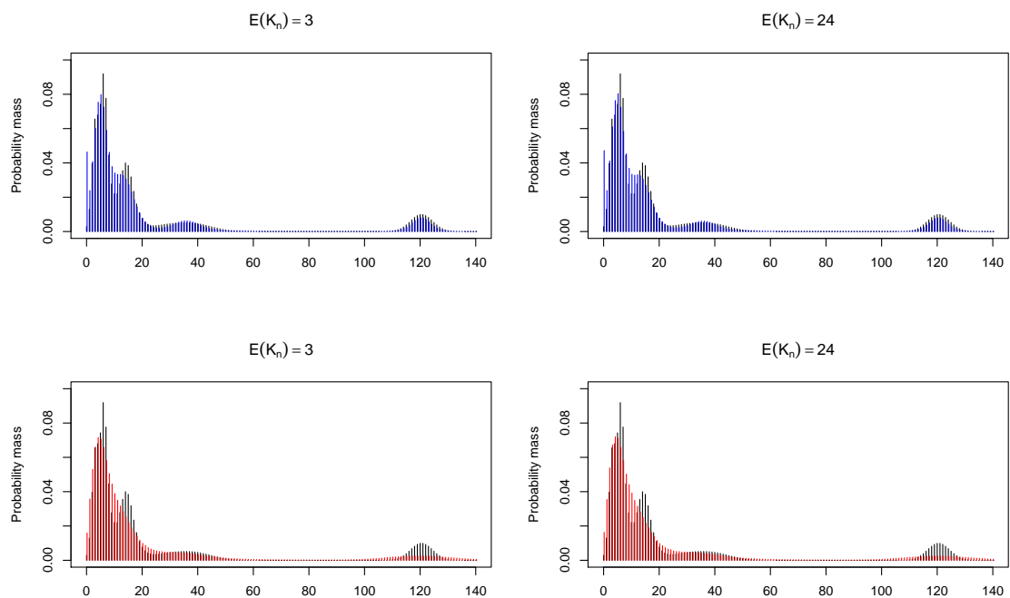
Figure 12. Posterior probability mass functions given n = 100 data generated from the 12 component RG mixture. The first row displays the posterior estimates of the RG model (depicted in solid blue) whereas the second of the Poisson model (depicted in solid red) both with \sigma = 0.75 and, respectively, \mathbb{E}[K_n] = 3 and \mathbb{E}[K_n] = 24 . The true pmf are in solid black.
