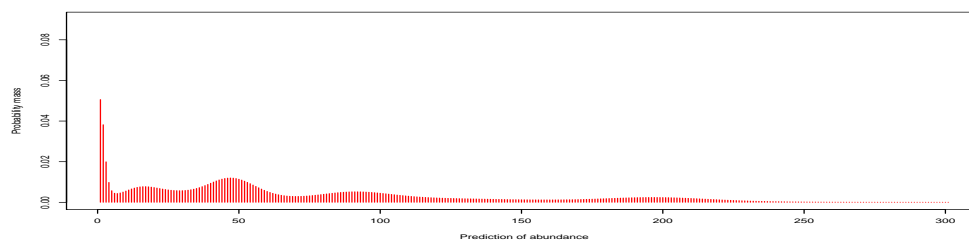
(c) \sigma = 0.5
