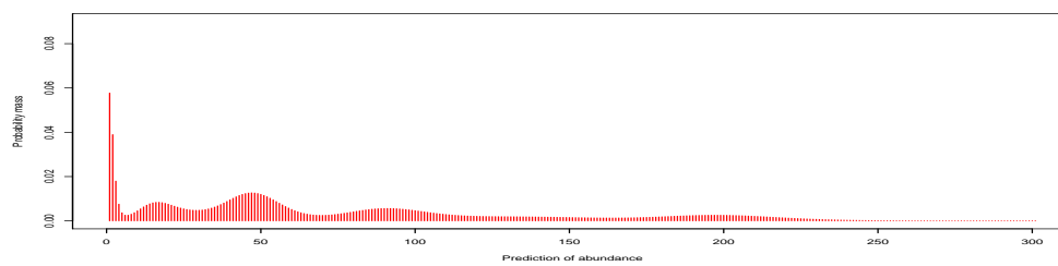
(a) \sigma = 0
