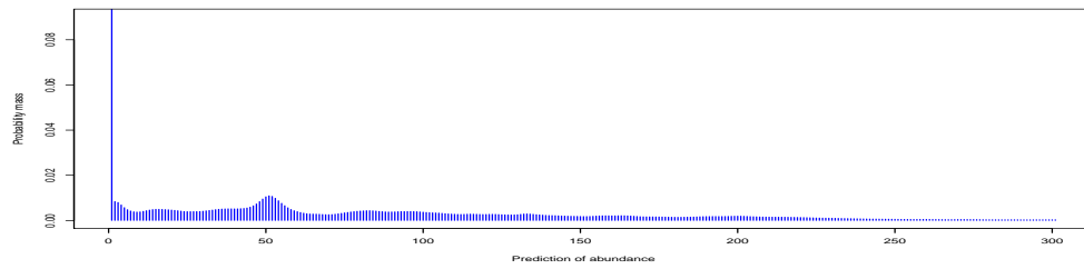
(c) \sigma = 0.5
