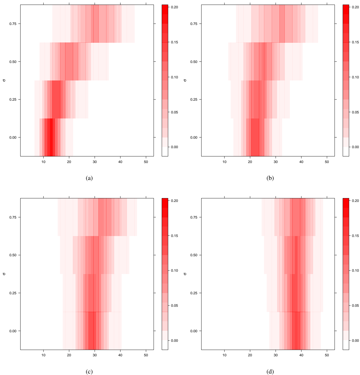
Figure 2. Posterior distributions of the number of components K_n — for the Okaloosa darters dataset for the Poisson mixture model as \sigma varies. The prior expected number of components \mathbb{E}[K_n] is set equal to 10 (a), 22 (b), 30 (c), and 40 (d). The posterior probability mass is represented with a color scale ranging from white for low probability to darker color for higher probability.
