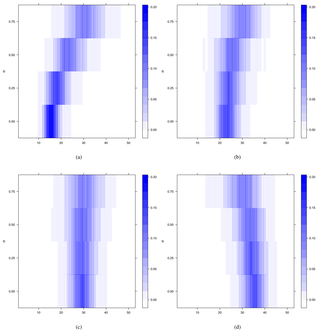
Figure 1. Posterior distributions of the number of components K_n — for the Okaloosa darters dataset for the RG mixture model as \sigma varies. The prior expected number of components \mathbb{E}[K_n] is set equal to 10 (a), 22 (b), 30 (c), and 40 (d). The posterior probability mass is represented with a color scale ranging from white for low probability to darker color for higher probability.
