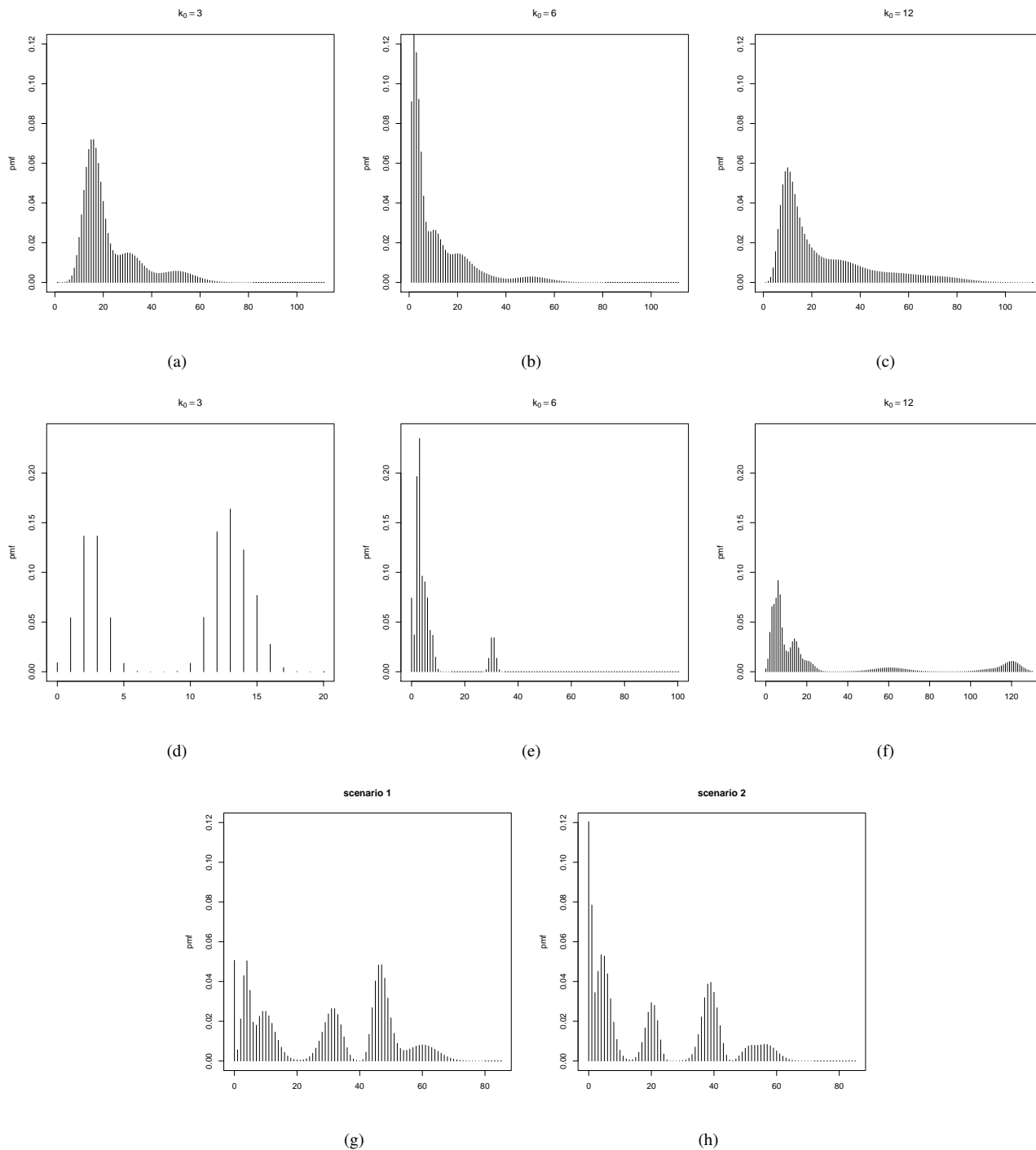
Figure 11. Data generating pmf for the simulation experiments of Section 3. The pmf in the first row correspond to Poisson mixtures with k_0 = 3, 6, 12 components, the pmf in the second row to RG mixtures with k_0 = 3, 6, 12 components and the third row to the complex mixtures described in, respectively, (9) and (10).
