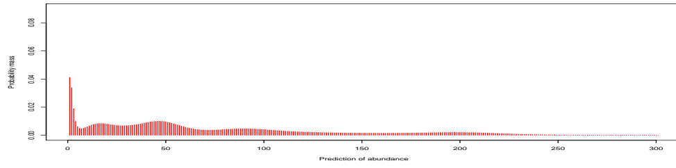
(a) \sigma = 0
