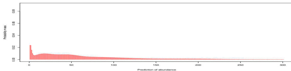
(c) \sigma = 0.5
