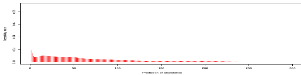
(b) \sigma = 0.25
