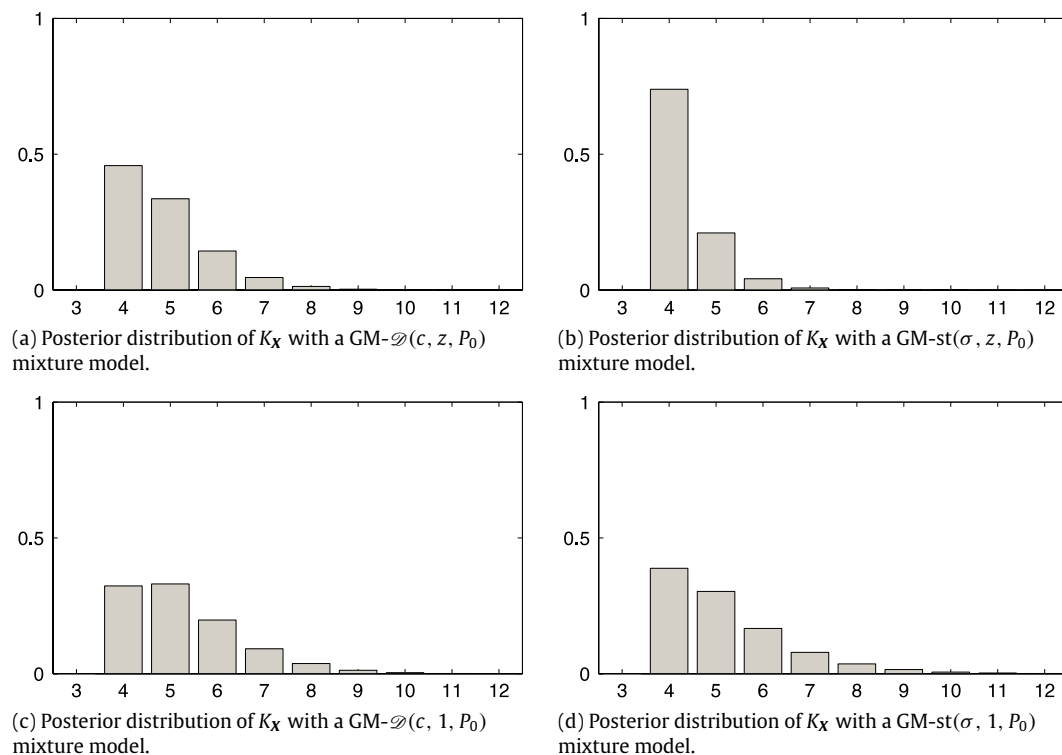
Fig. 5. (Example 1) GM- \mathcal{D} and GM-st mixtures (top row) vs. two independent univariate Dirichlet and normalized \sigma -stable process mixtures (bottom row): posterior distributions of the number of clusters for the first sample.
