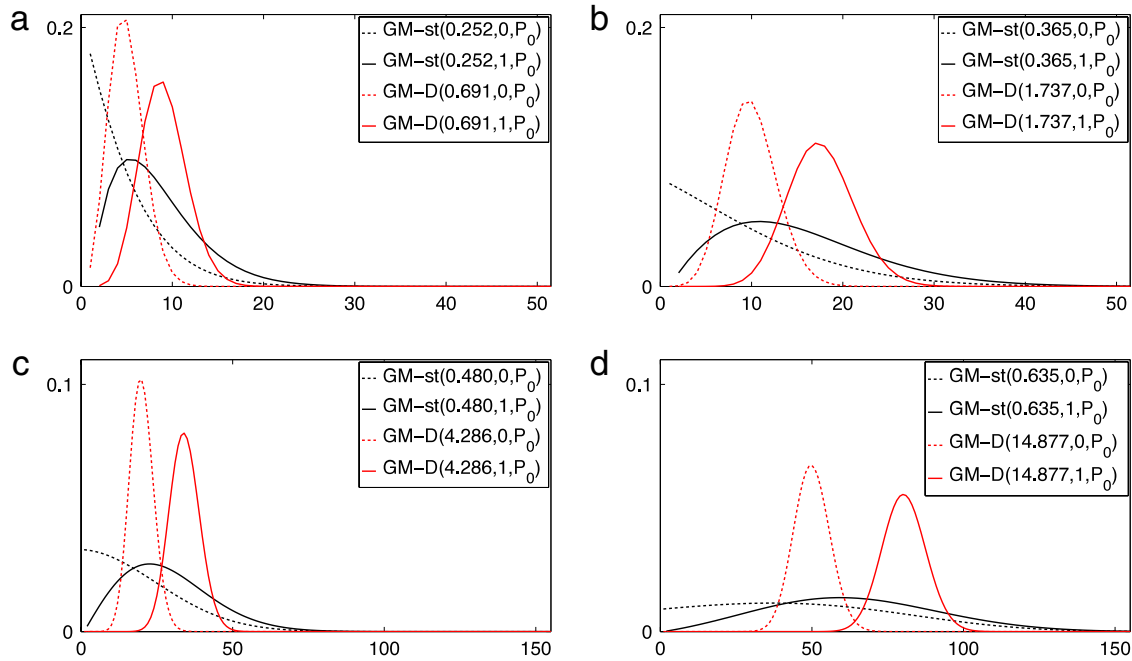
Fig. 1. Prior distribution of the number of clusters of two samples of sizes n_1 = n_2 = 200 governed by GM- \mathcal{D} processes (red lines) or GM-st processes (black lines) in the two extreme cases of z = 0 (dashed lines) and z = 1 (solid lines). The parameters c and \sigma are chosen so that, with z = 0 , the expected number of clusters is approximately equal to 5 in (a), 10 in (b), 20 in (c) and 50 in (d).
