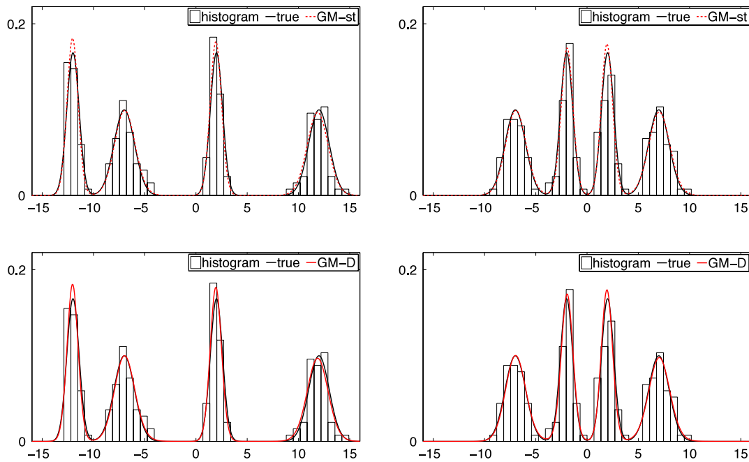
Fig. 4. (Example 1) True data generating densities ( f_1 on the left column and f_2 on the right column) with histograms of the simulated data. Corresponding estimates are obtained with the GM-st( \sigma, Z, P_0 ) mixture model (first row) and the GM- \mathcal{D} ( c, Z, P_0 ) mixture model (second row).
