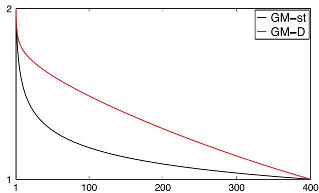
Fig. 2. Plot of the ratio \mathbb{E}[K_{n_1+n_2}^{(1)}] / \mathbb{E}[K_{n_1+n_2}^{(0)}] , as a function of \mathbb{E}[K_{n_1+n_2}^{(0)}] , for mixture models based on GM- \mathcal{D} and GM-st processes, with n_1 = n_2 = 200 .
