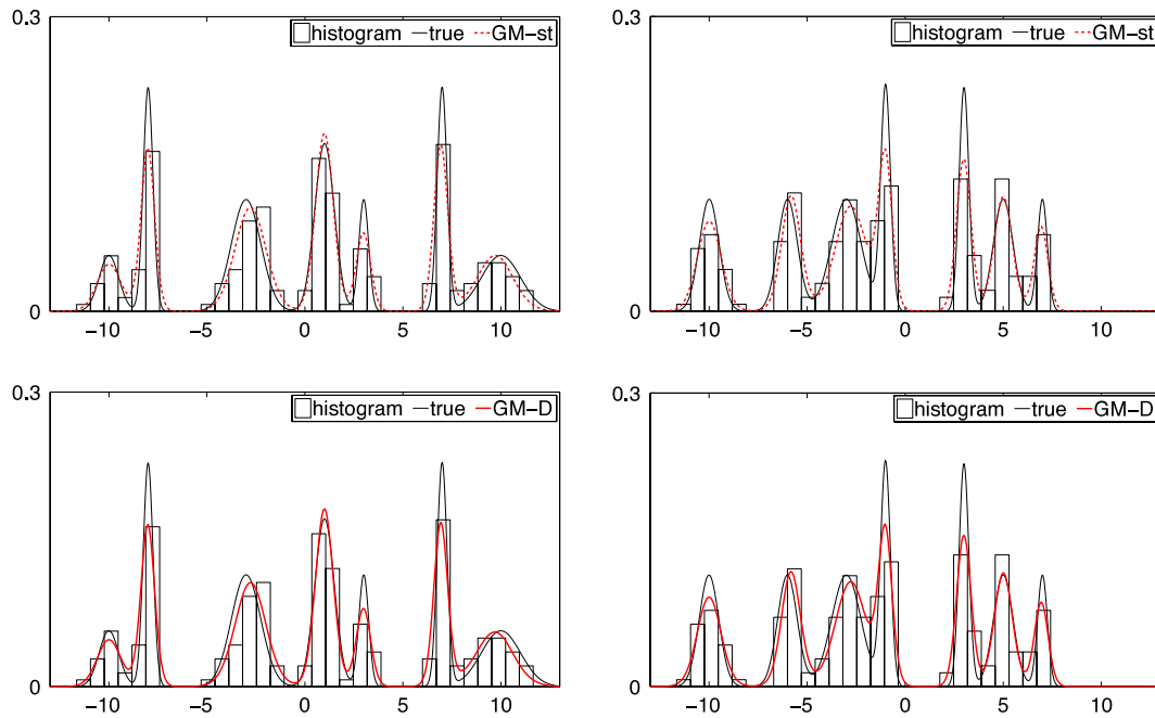
Fig. 6. (Example 3) True data generating densities ( f_1 on the left column and f_2 on the right column) with histograms of the simulated data. Corresponding estimates are obtained with the GM-st( \sigma, Z, P_0 ) mixture model (first row) and the GM- \mathcal{D}(c, Z, P_0) mixture model (second row).
