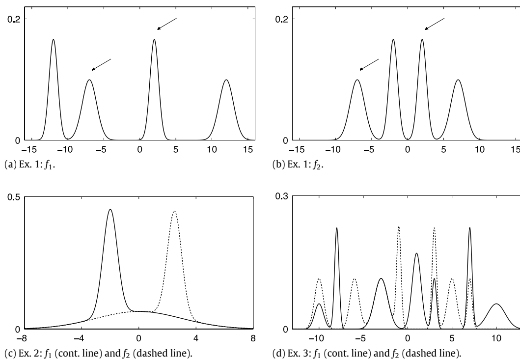
Fig. 3. (Examples 1–3) True densities f_1 and f_2 generating the simulated datasets.
