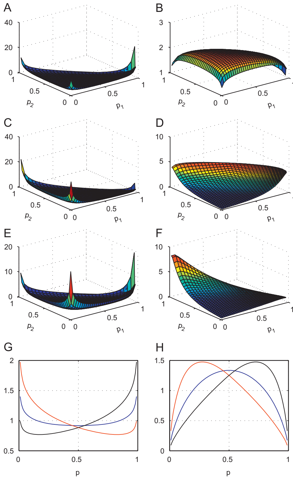
Fig. 2. NID distribution based on gamma r.v. with different scale and shape parameters: (A) On \Delta^{(2)} with \alpha_i = 0.5790 , \gamma_i = 1 , i = 1, 2, 3 . (B) On \Delta^{(2)} with \alpha_i = 1.09 , \gamma_i = 1 , i = 1, 2, 3 . (C) On \Delta^{(2)} with \alpha_i = 0.5790 , i = 1, 2, 3 , \gamma_1 = 3 , \gamma_2 = \gamma_3 = 1 . (D) On \Delta^{(2)} with \alpha_i = 1.09 , i = 1, 2, 3 , \gamma_1 = \gamma_2 = 1 , \gamma_3 = 1 . (E) On \Delta^{(2)} with \alpha_i = 0.5790 , i = 1, 2, 3 , \gamma_1 = \gamma_2 = 3 , \gamma_3 = 2 . (F) On \Delta^{(2)} with \alpha_i = 1.09 , i = 1, 2, 3 , \gamma_1 = 2 , \gamma_2 = 1 , \gamma_3 = 3 . (G) On (0,1) with \alpha_i = 0.8685 , i = 1, 2 , \gamma_i = 1 , i = 1, 2 , (blue), with \alpha_i = 0.8685 , i = 1, 2 , \gamma_1 = 3 , \gamma_2 = 2 (red) and with \gamma_1 = 2 , \gamma_2 = 3 (black). (H) On (0,1) with \alpha_i = 1.6350 , i = 1, 2 (blue), with \alpha_i = 1.6350 , i = 1, 2 , \gamma_1 = 3 , \gamma_2 = 2 (red) and with \gamma_1 = 2 , \gamma_2 = 3 (black). (For interpretation of the references to color in this figure legend, the reader is referred to the web version of this article.)
