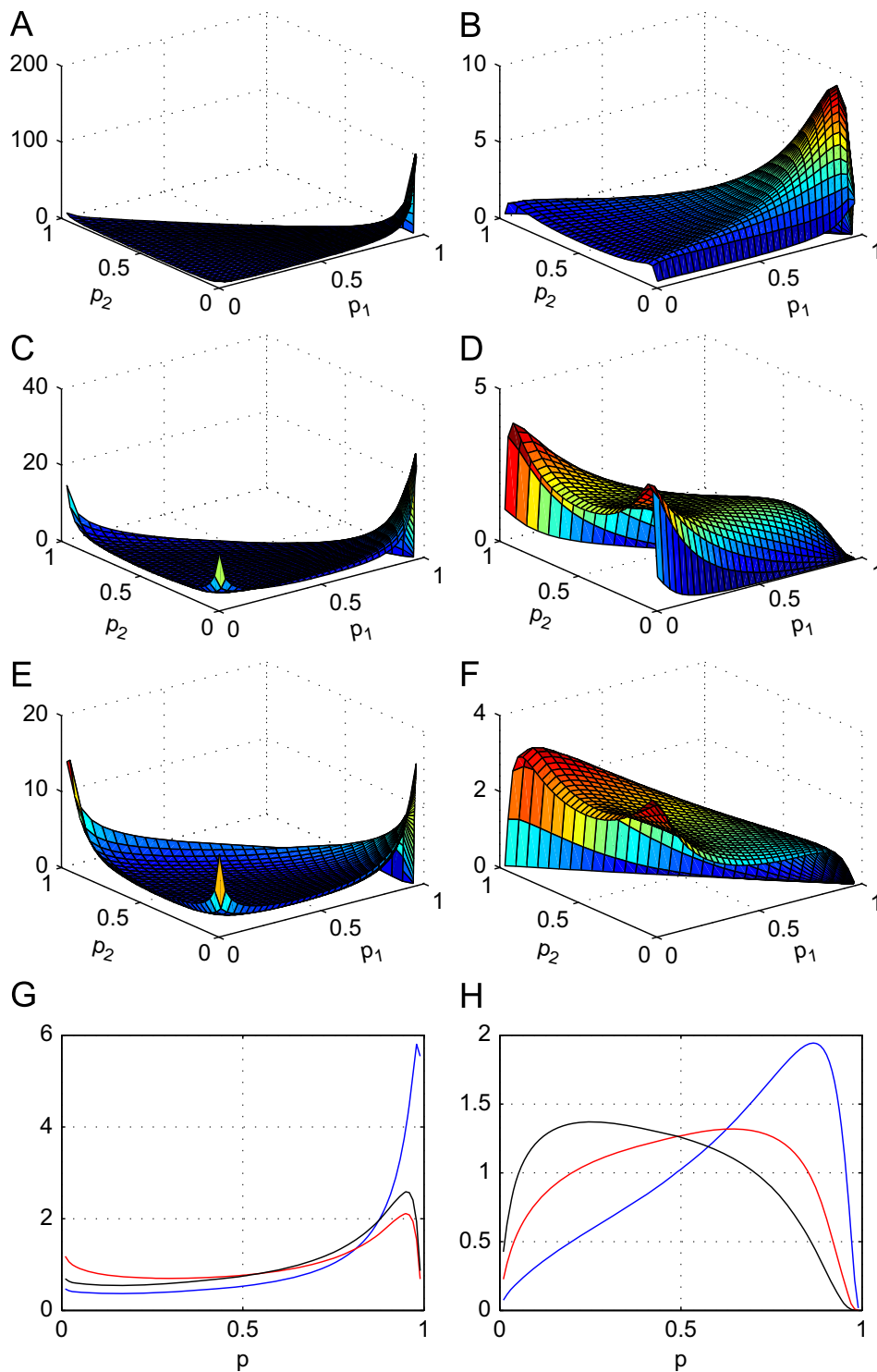
Fig. 1. NID distribution based on gamma and inverse-Gaussian r.v.: (A) On \Delta^{(2)} with \alpha_1 = 0.5790 , \gamma_1 = 1 , \lambda_i = 0.1667 , \theta_i = 1 , i = 1, 2 . (B) On \Delta^{(2)} with \alpha_i = 1.09 , \gamma_1 = 1 , \lambda_i = 0.6 , \theta_i = 1 , i = 1, 2 . (C) On \Delta^{(2)} with \alpha_1 = 0.5790 , \gamma_1 = 3 , \lambda_i = 0.1667 , \theta_i = 1 , i = 1, 2 . (D) On \Delta^{(2)} with \alpha_1 = 1.09 , \gamma_1 = 3 , \lambda_i = 0.6 , \theta_i = 1 , i = 1, 2 . (E) On \Delta^{(2)} with \alpha_i = 0.5790 , \gamma_i = 3 , i = 1, 2 , \lambda_1 = 0.1667 , \theta_1 = 1 . (F) On \Delta^{(2)} with \alpha_i = 1.09 , \gamma_i = 3 , i = 1, 2 , \lambda_1 = 0.6 , \theta_1 = 1 . (G) On (0, 1) with \alpha_1 = 0.8685 , \lambda_1 = 0.25 , \gamma_1 = 1 , \theta_1 = 1 (blue), \gamma_1 = 3 , \theta_1 = 1 (red) and with \gamma_1 = 3 , \theta_1 = 2 (black). (H) On (0, 1) with \alpha_1 = 1.6350 , \lambda_1 = 0.9 , \gamma_1 = 1 , \theta_1 = 1 (blue), \gamma_1 = 2 , \theta_1 = 1 (red) and with \gamma_1 = 3 , \theta_1 = 1 (black). (For interpretation of the references to color in this figure legend, the reader is referred to the web version of this article.)
