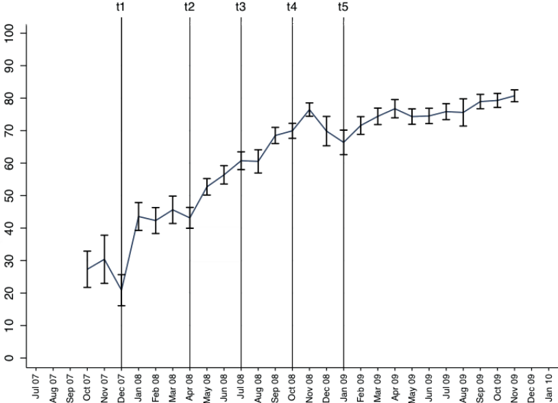
Figure 5: Average Compliance
