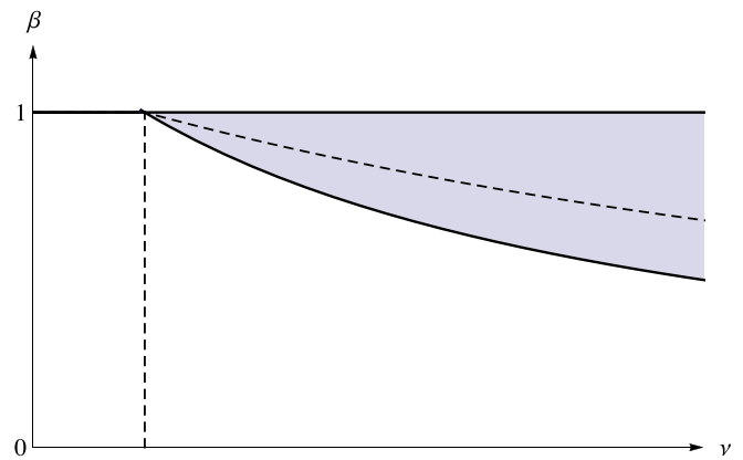
Fig. 1. The region where mergers are pro-competitive. Condition (6) holds to the right of the dashed vertical line, and condition (7) holds in the grey area. The dashed curve separates the regions where the post-merger equilibrium is interior (above the curve) or involves a corner solution x_M = c (below the curve). The figure has been drawn for c = 0.3 and n = 4 .
