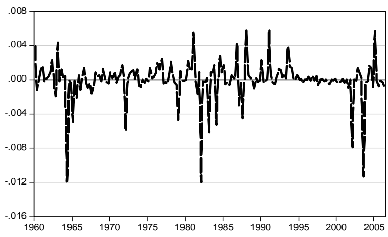
Figure 4. Assessing the R&R robustness check
