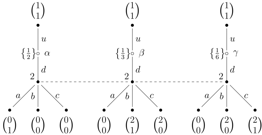
Figure 1: A signaling game.
