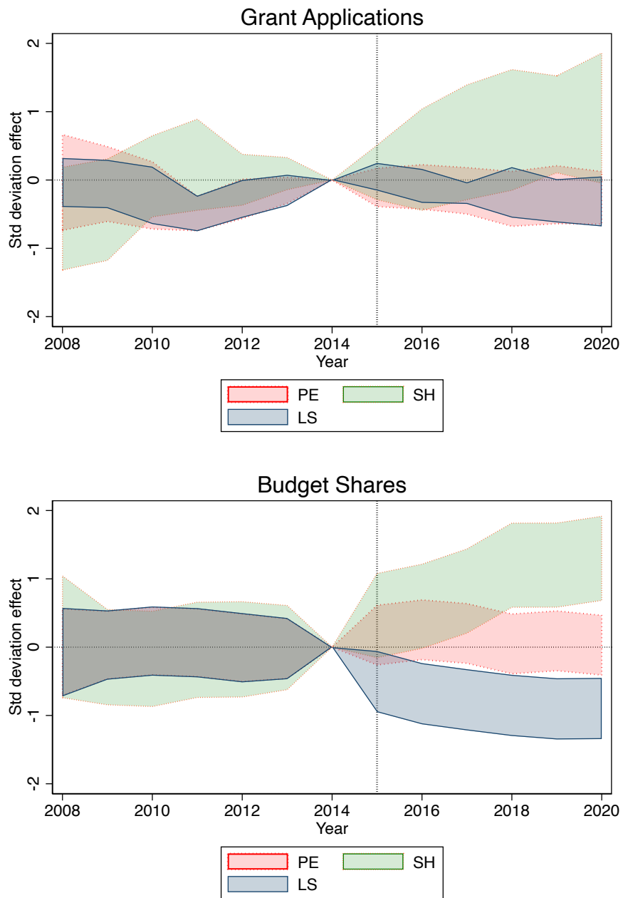
FIGURE XV: Event Analysis
