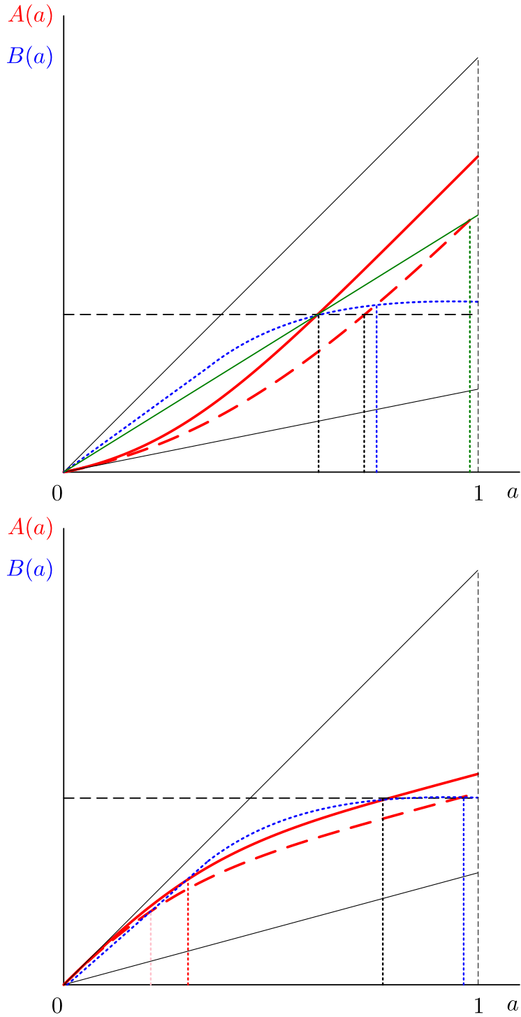
FIGURE V: Comparative Statics
