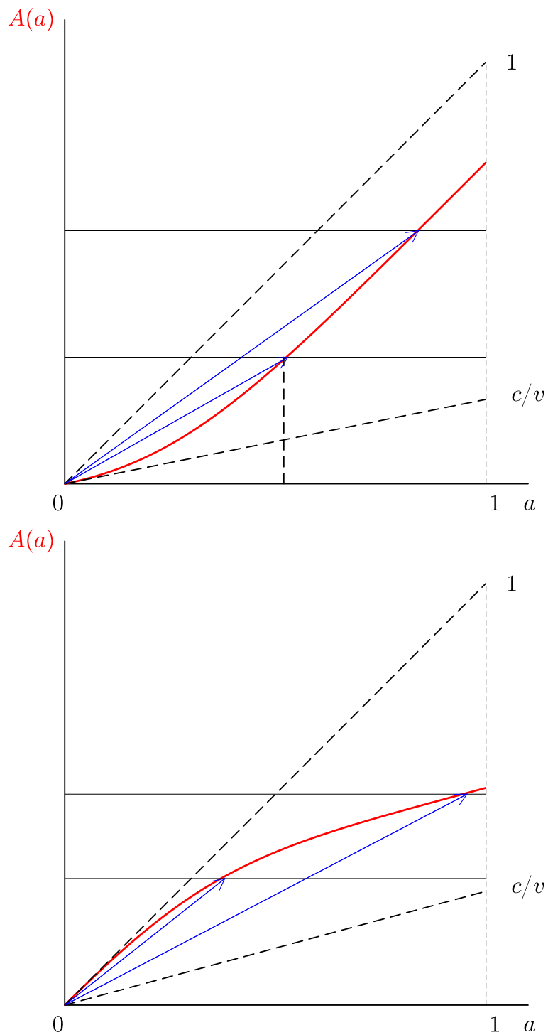
FIGURE IV: Award Function
