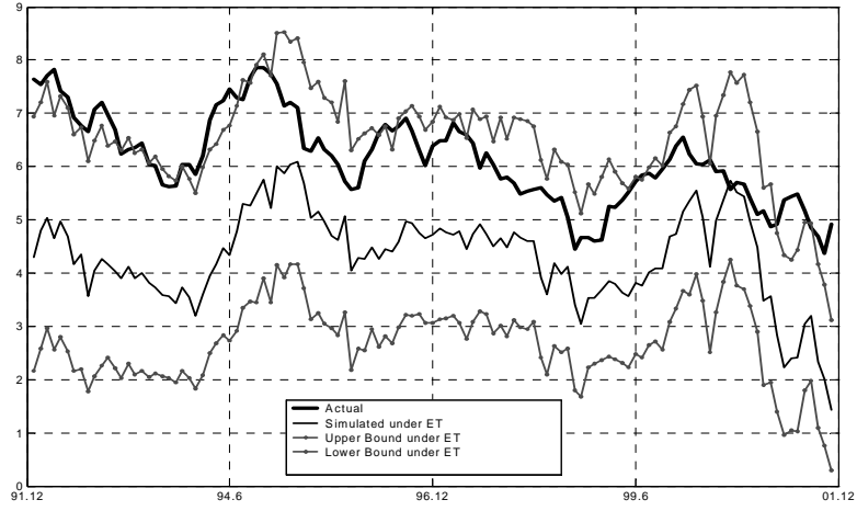
Figure 4: Simulated ET-consistent 10-year yields to maturity based on the CS model, with lower and upper bond of its 90% Confidence Interval
