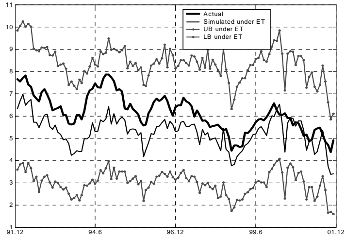
Figure 6: Simulated ET-consistent 10-year yields to maturity based on the model with financial factors and macroeconomic variables, with lower and upper bound of its 90% Confidence Interval
