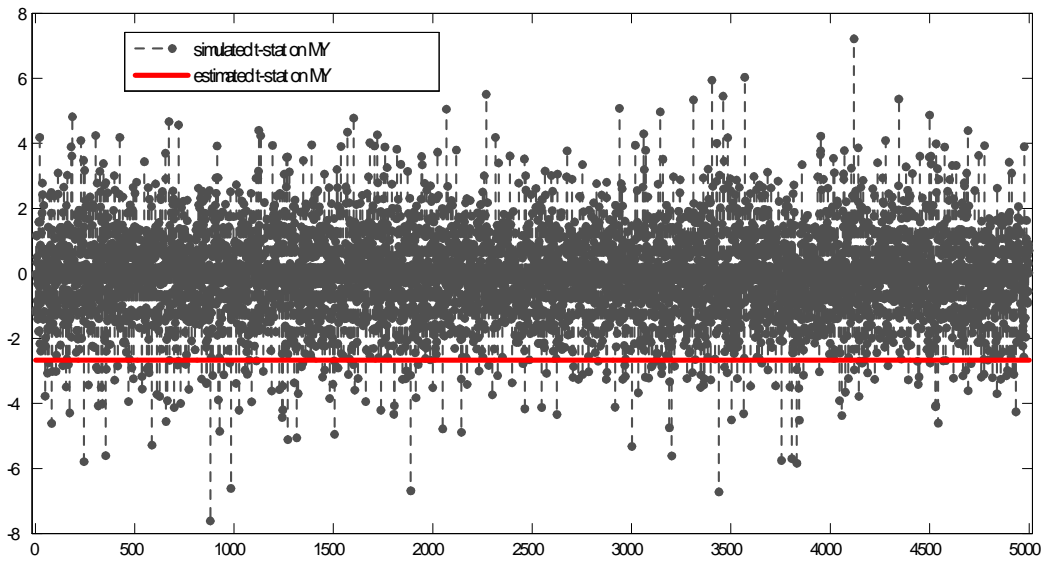
Figure 7.1. Simulated vs. estimated t-statistics, real 3-month yield.
