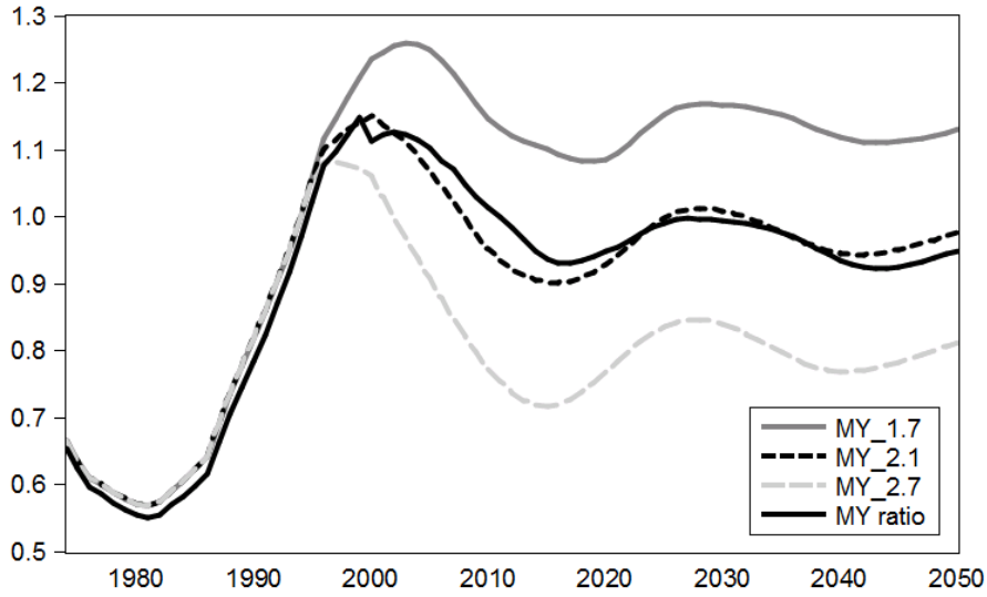
Figure 6.1. MY projections and fertility rates.
