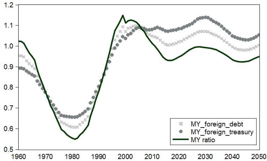
Figure 6.2. MY projections and foreign holdings.
