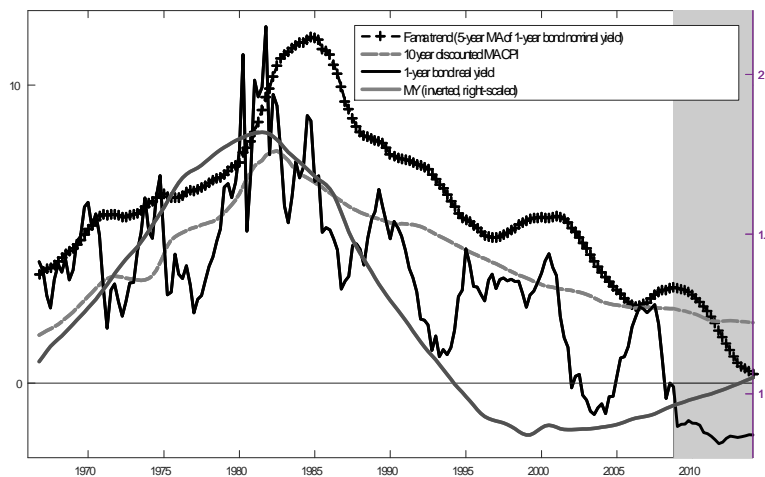
Figure 2.2. 1-Year US Treasury bond real yields and the permanent component.
