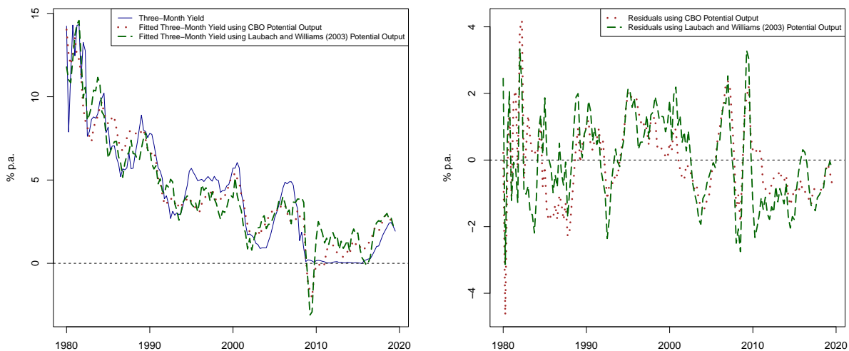
(b) Residual u_t^{(1)} from policy rules.
