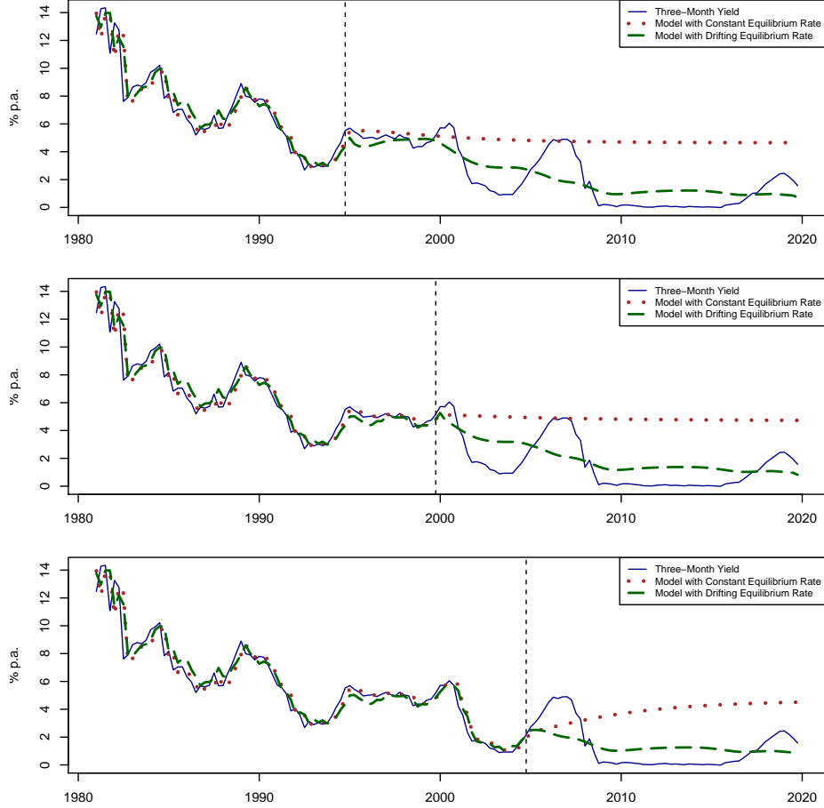
Figure 2: Long-Term Forecasts of Short-Term Rate. This figure shows actual three-month yield and predicted rates implied by our (cointegrated) model with drifting equilibrium rates (c.f. equation (2); green dashed line) and by a model that restricts the equilibrium rate to be constant (c.f. equation (3); brown dotted line). The forecast of the drifting rule exploits the exogeneity of the demographic variable ( MY ) and of potential output ( \Delta x^{pot} ). In particular, the rule is estimated until 1995, 2000, and 2005 in the top, mid, and bottom panels, respectively. We then use the coefficients estimates, the projections of MY and \Delta x^{pot} (see also Appendix A), and the forecast of inflation and output gap from a VAR(1) as in equations (7) and (8). \pi^* is modeled as a random walk. Monetary policy residuals persistence \rho is 0.673 and 0.949 for the drifting and the constant equilibrium rate models respectively. Dotted vertical lines represent the end of in-sample estimation period. Quarterly observations. The sample period is 1980:Q1 to 2019:Q4.
