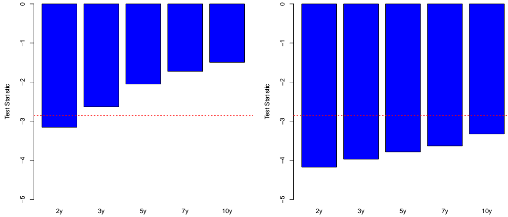
(a) Model with constant equilibrium rate. (b) Model with drifting equilibrium rate.
