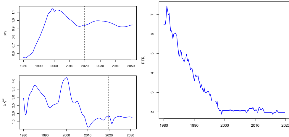
Figure A.1: Drivers of the Equilibrium Nominal Rate. This figure shows the dynamics for the drivers of the time-varying equilibrium nominal rate y_t^* in equation (2). The left panel shows the ratio of middle-aged (40-49) to young (20-29) population, MY , and for potential output growth, \Delta x_t^{pot} . The right panel shows the Federal Reserve’s perceived target rate (PTR) for inflation. MY is available until 2050 and is hand-collected from various past Census reports available at https://www.census.gov/data.html . Potential output is available until 2030 and can be downloaded at https://fred.stlouisfed.org/series/GDPPOT . Dotted vertical lines denote the end of our sample, i.e., 2019:Q4. Quarterly observations.
