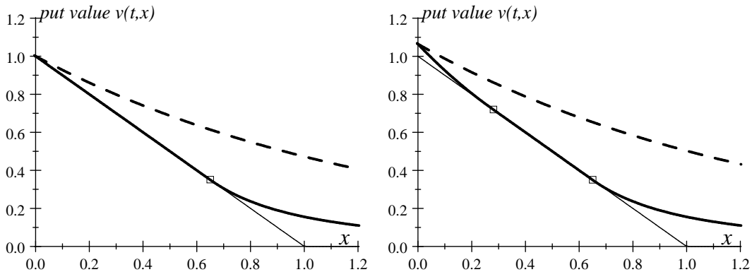
Finite-maturity put value with \rho \geq 0 .
