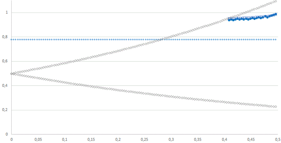
Figure 1. The free boundary when r_d is positive. The grey diamonds delimit the stock binomial tree. Blue dots denote the binomial free boundary, and blue stars its asymptotic approximation. Blue circles denote the perpetual boundary.
